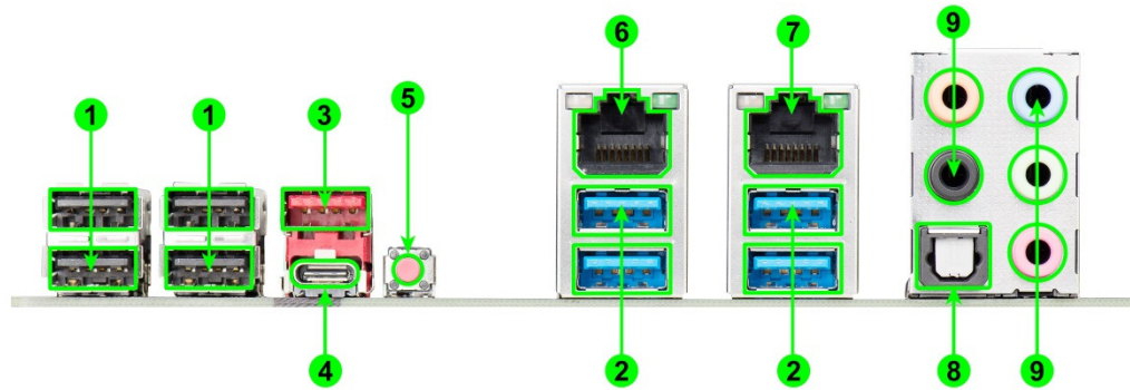
Figure 2. Chassis Rear Panel Connectors
